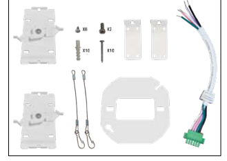
SB-OL-SMK-WMK-W Wall and Surface Mounting KIT Wire Rope Length:φ0.04X4.7 inch (2PCS) Wire Length : 7.9 inches (2FT,4FT,8FT)
