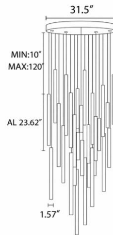
SB-R135A180W/35 Lights
