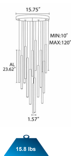
SB-R115A80W/15 Lights
