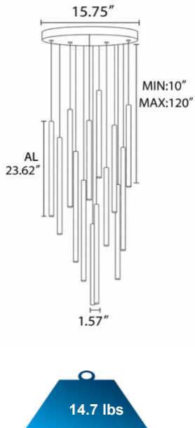
SB-R112A60W/12 Lights
