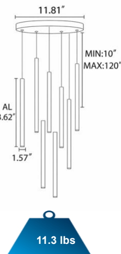
SB-R108A40W/8 Lights
