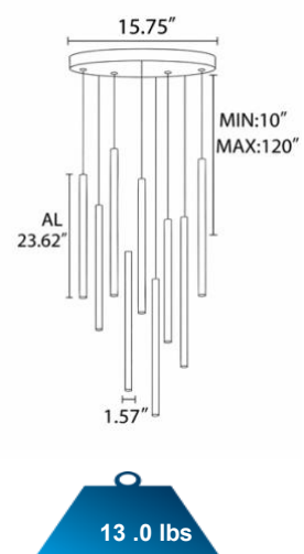
SB-R110A50W/10 Lights
