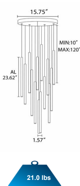
SB-R118A90W/18 Lights
