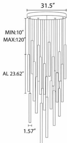
SB-R125A125W/25 Lights
