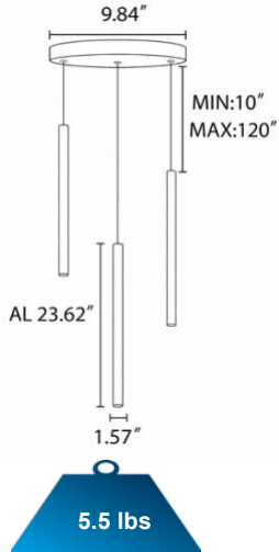
SB-R103A15W/3 Lights
