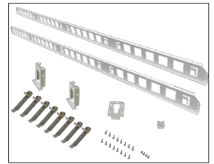
SB-8FT-OL-RMK-G2 Recessed Mounting Kit For 8FT Architecture Selectable LED Linear Light
