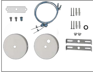
SB-OL-ceiling install Ceiling Install KIT Wire Rope Length: φ0.06X39.4-inch(2PCS)
